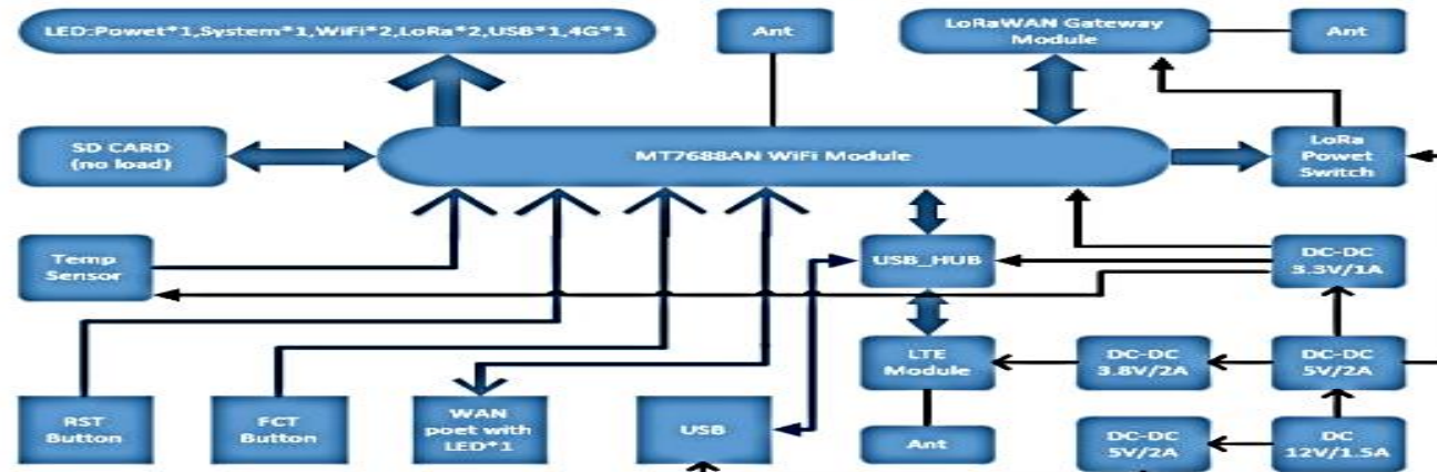
Figure 2-1 RHF2S025 functional block
